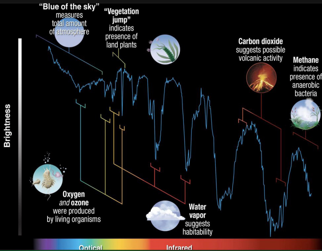
Figure 2.6 Earth's Spectrum
